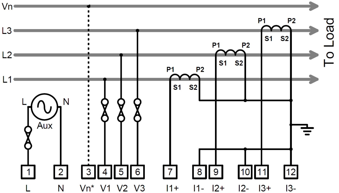
3-Phase 3 or 4-Wire (*Optional Neutral)
